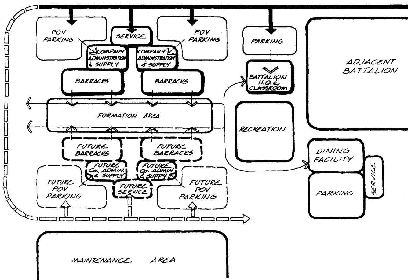
Figure 3-2. Functional Relationships Diagram for a Battalion Complex.
