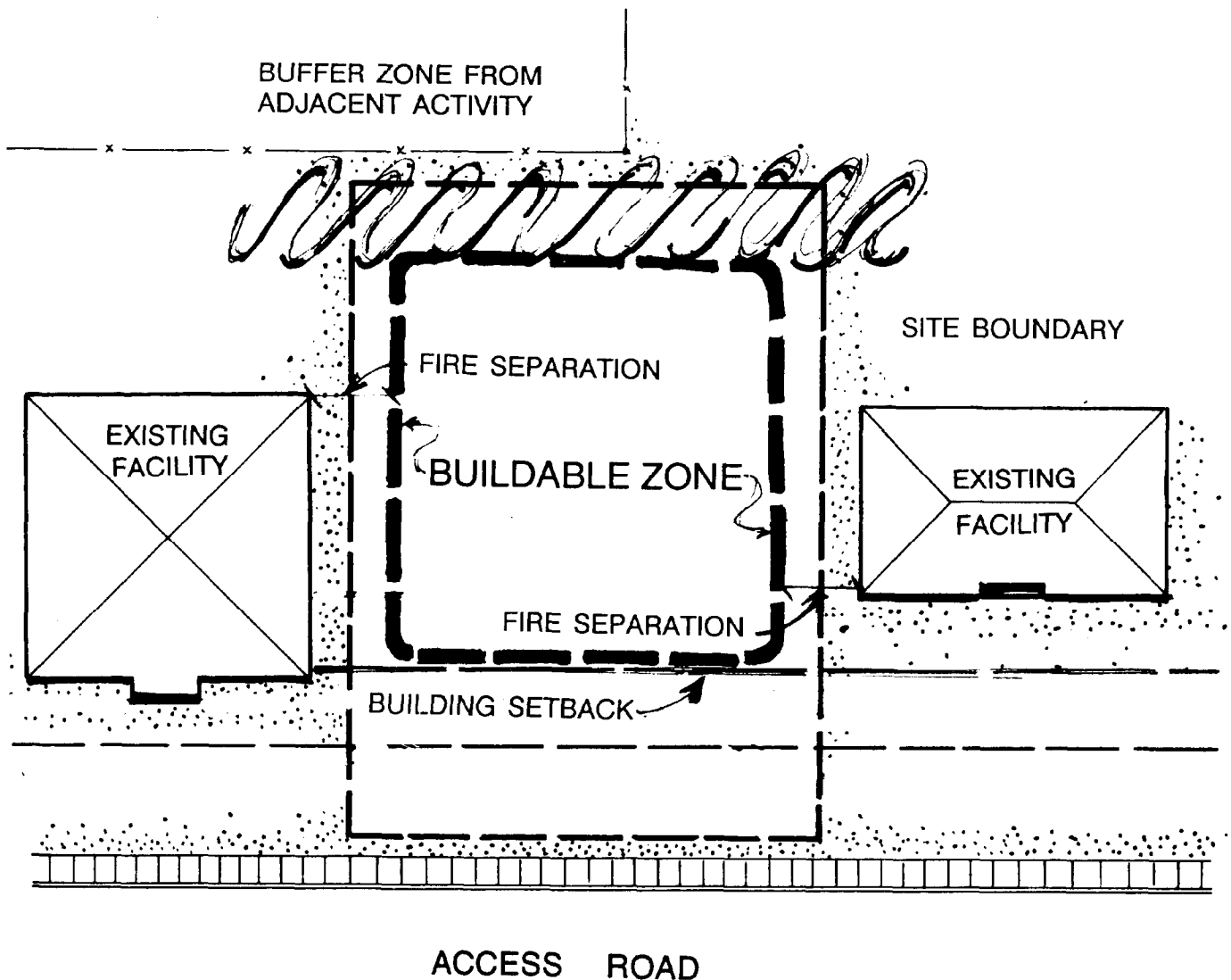
Figure 4-2. Buildable Zone.
