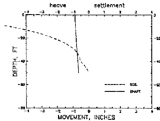
c. DISPLACEMENT-DEPTH BEHAVIOR, FILE MDEP
