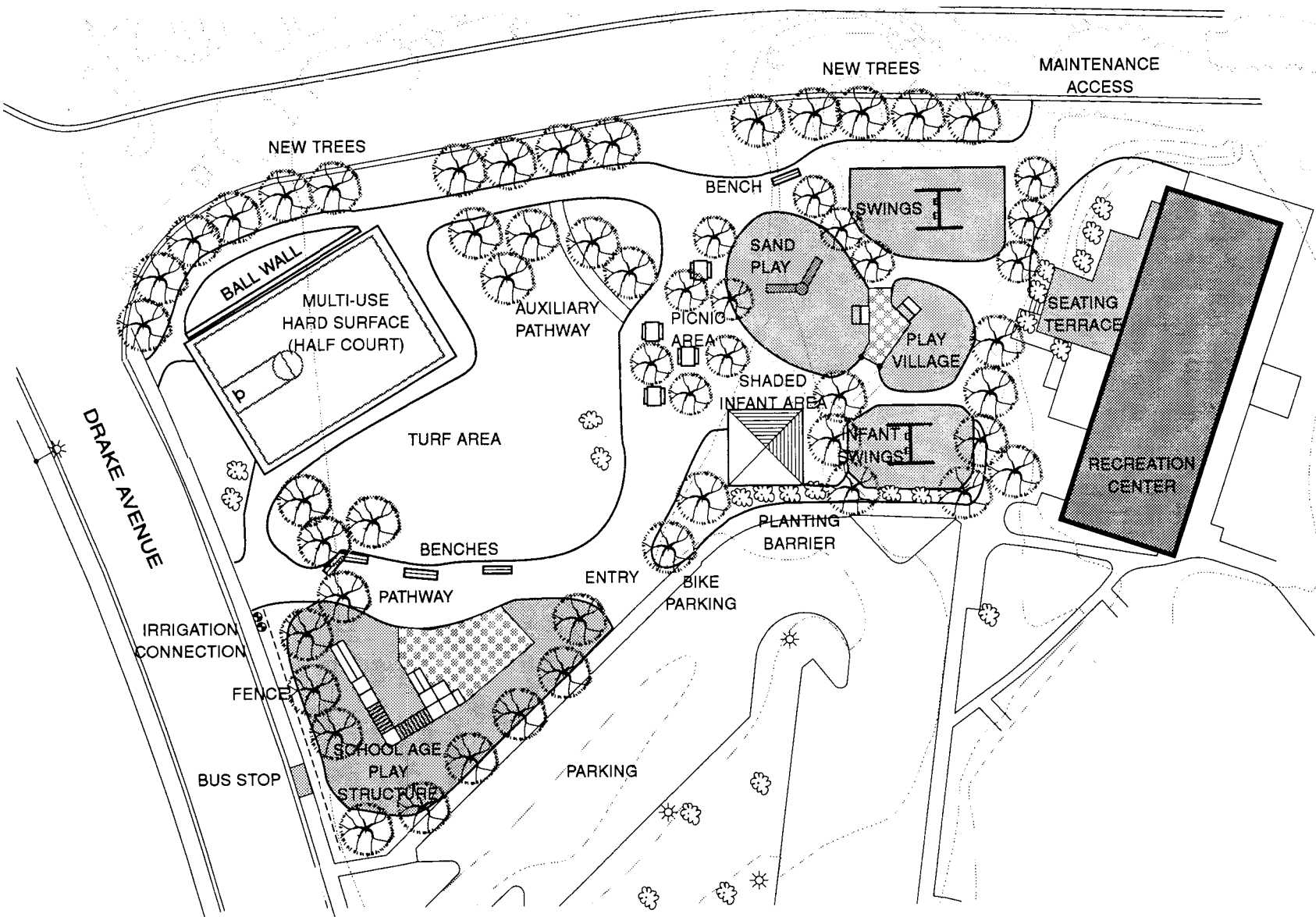
Figure 6-1 Conceptual Design
