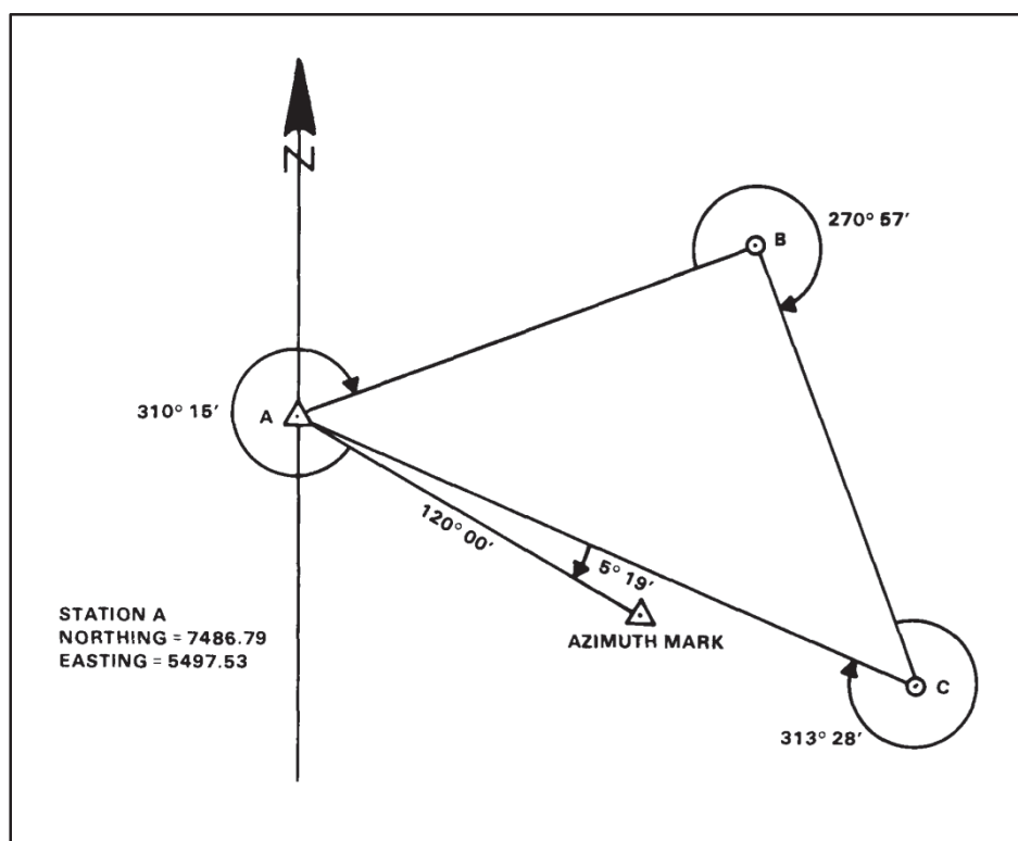
Figure 7-2. A loop traverse
