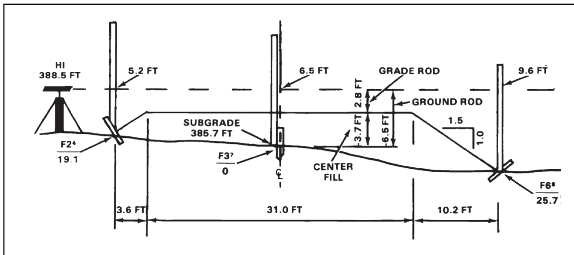
Figure 2-3. Marking slope stakes
