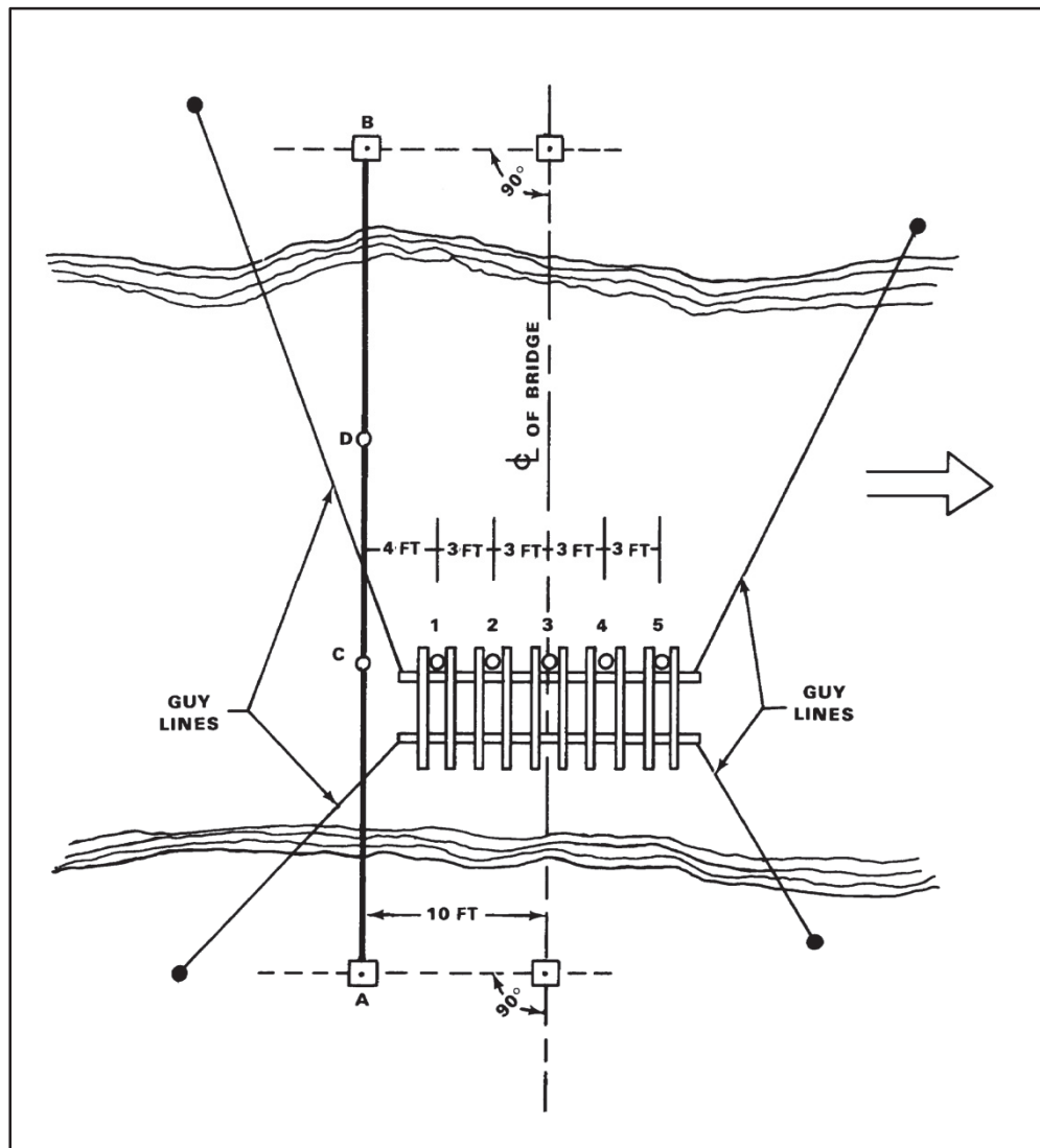
Figure 5-5. Positioning piles
