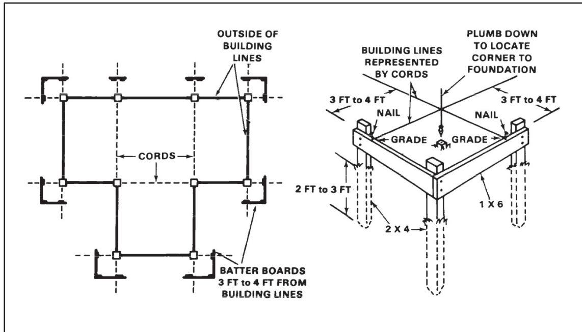
Figure 6-2. Batter boards
