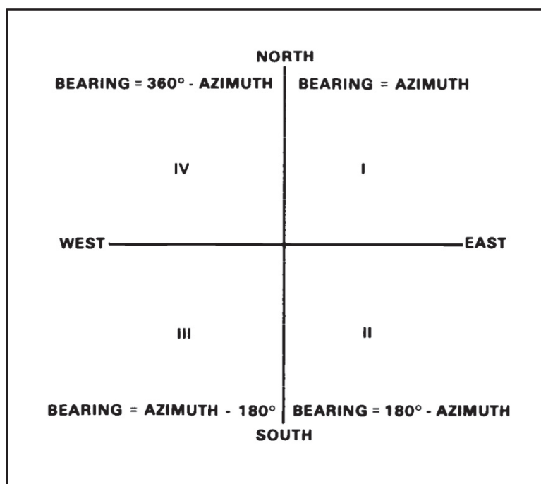
Figure 7-4. Determination of a bearing angle
