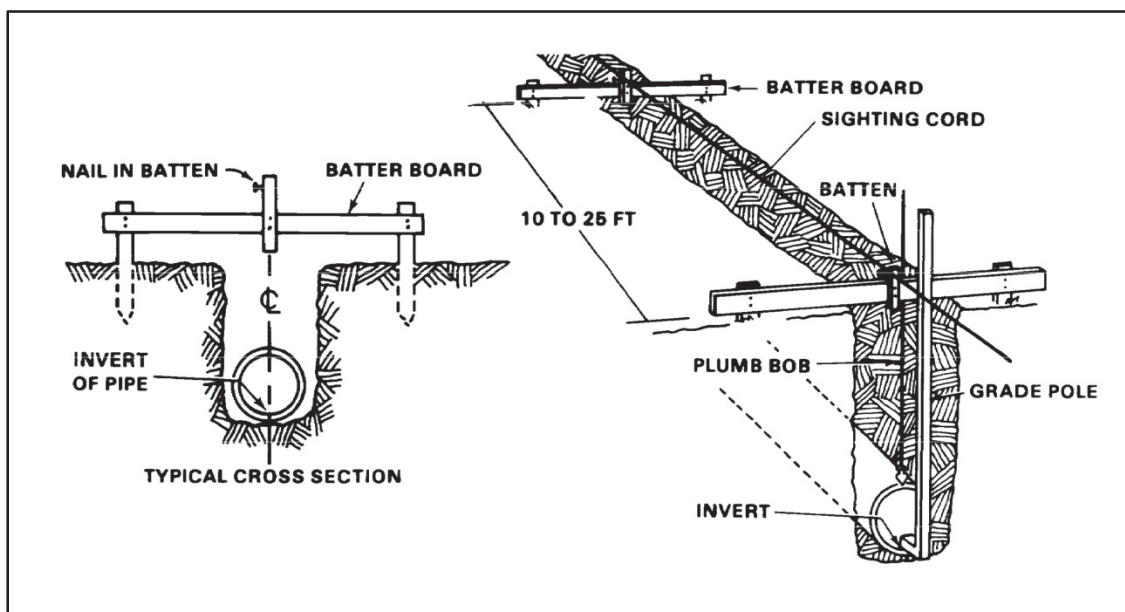
Figure 6-3. Sewer alignment
