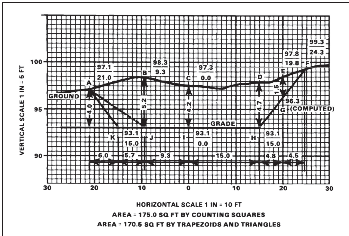
Figure 4-2. Area of irregular cross sections
