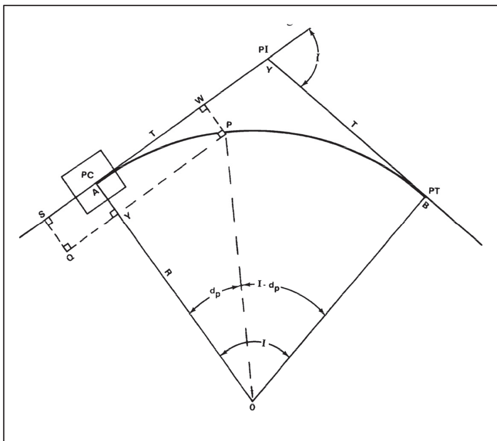
Figure 3-7. Inaccessible PC
