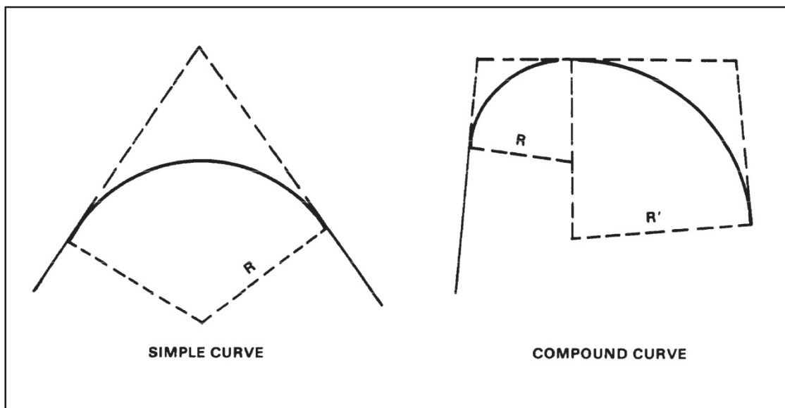
Figure 3-1. Horizontal curves
