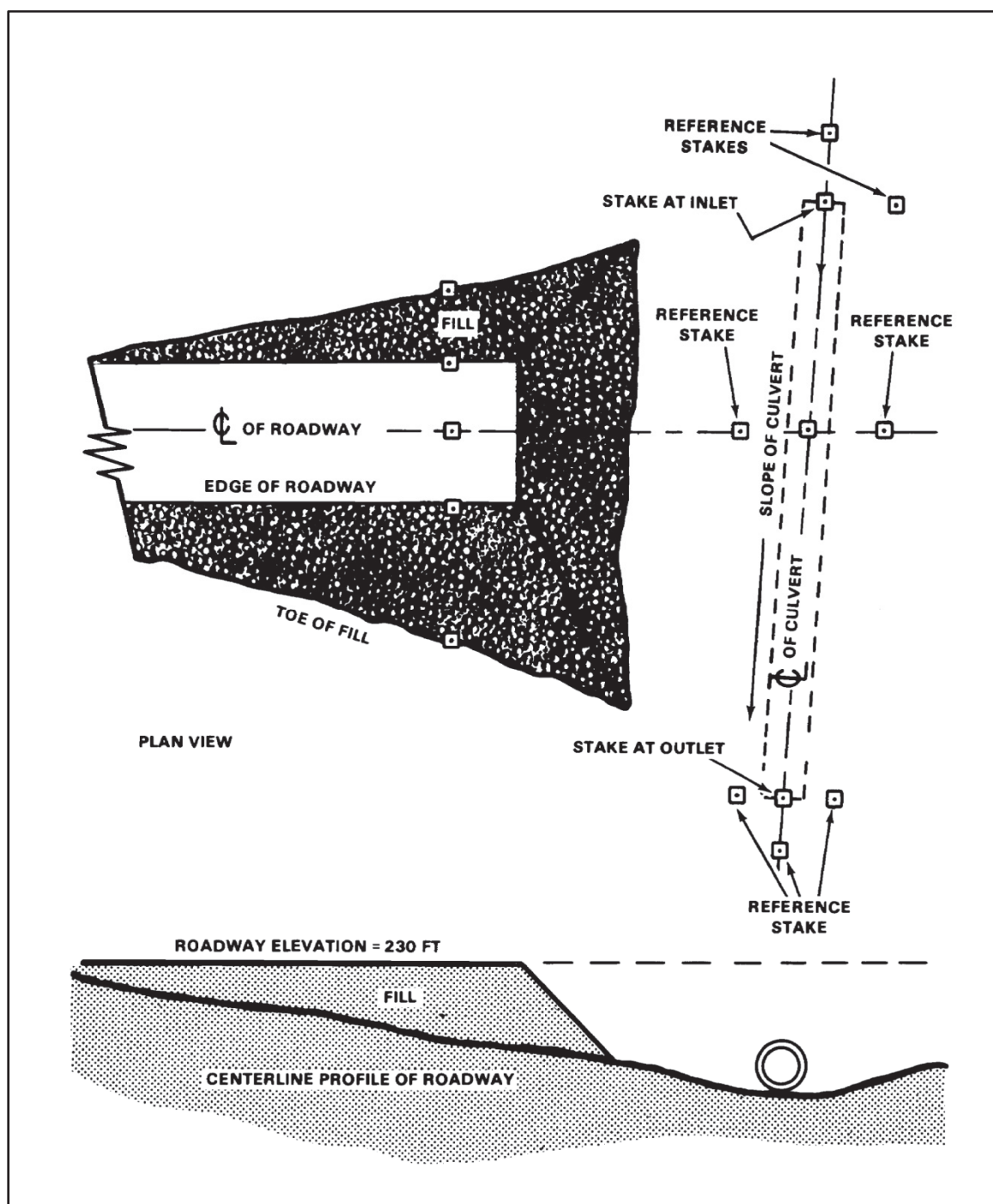
Figure 2-6. Layout of a culvert
