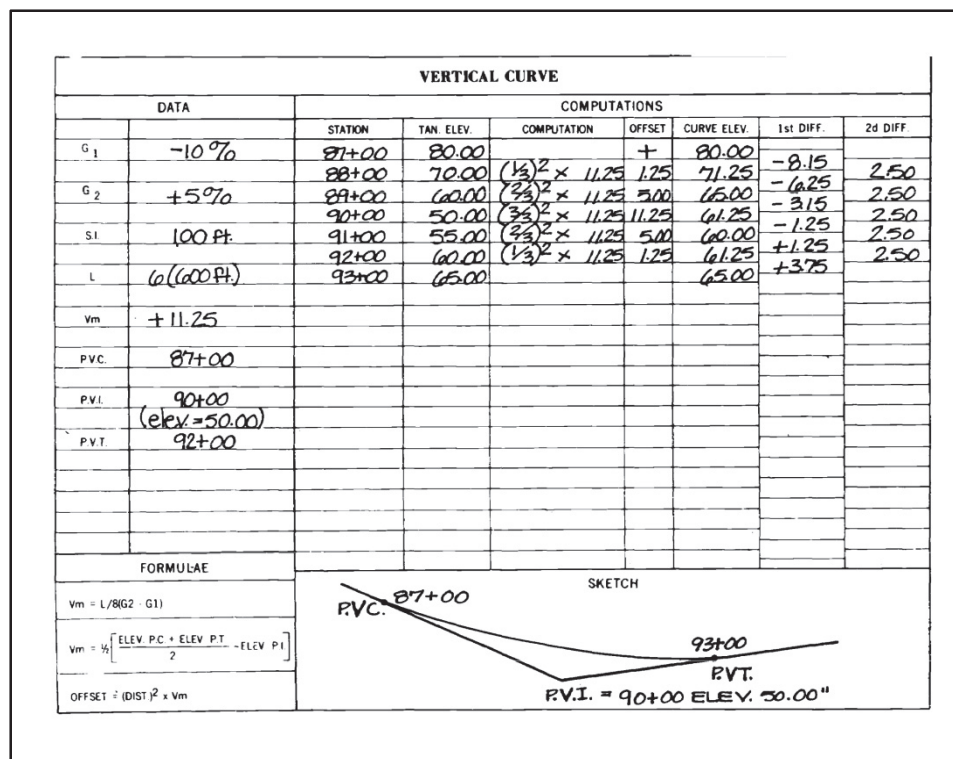
Figure 3-20. Typical solution of a sag curve
