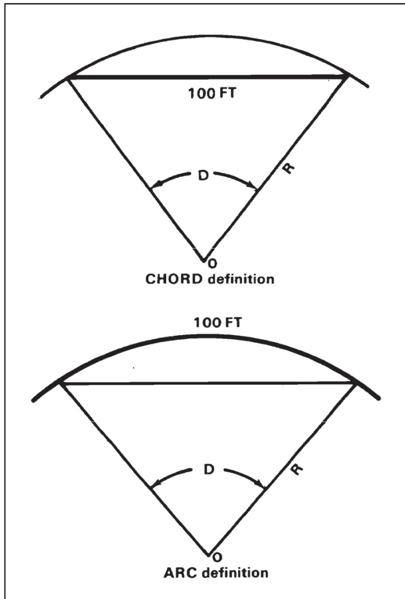
Figure 3-3. Degree of curve
