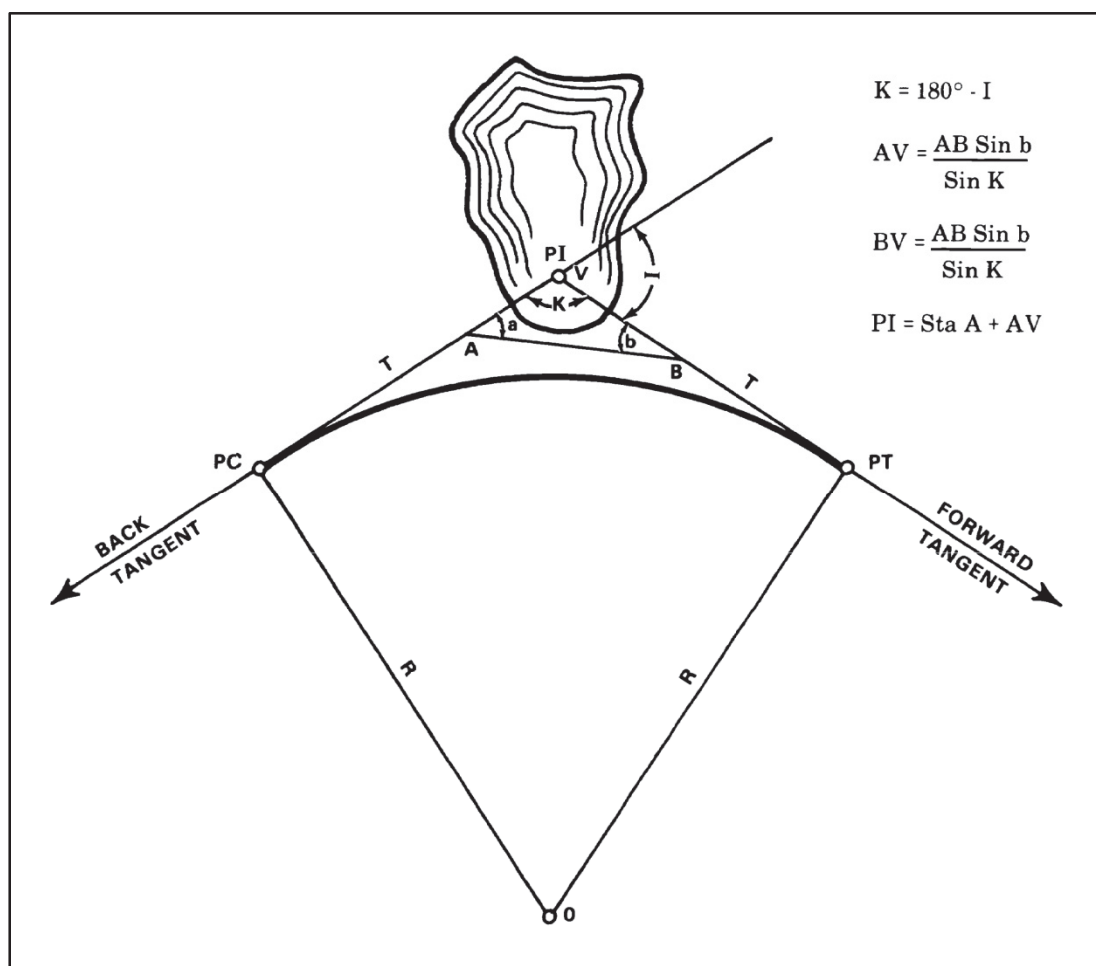
Figure 3-6. Inaccessible PI
