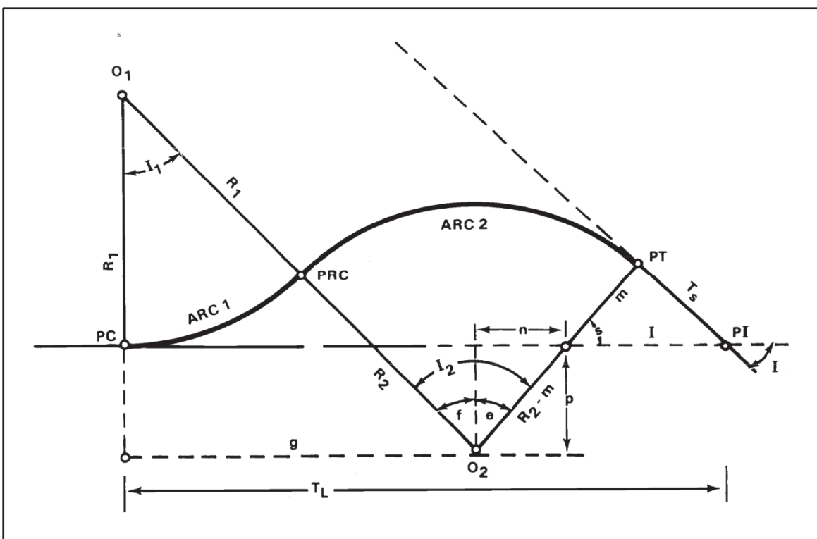
Figure 3-14. Reverse curve connecting diverging tangents
