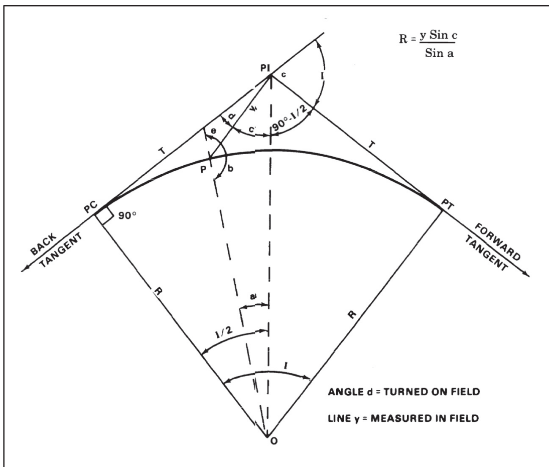
Figure 3-10. Curve through a fixed point
