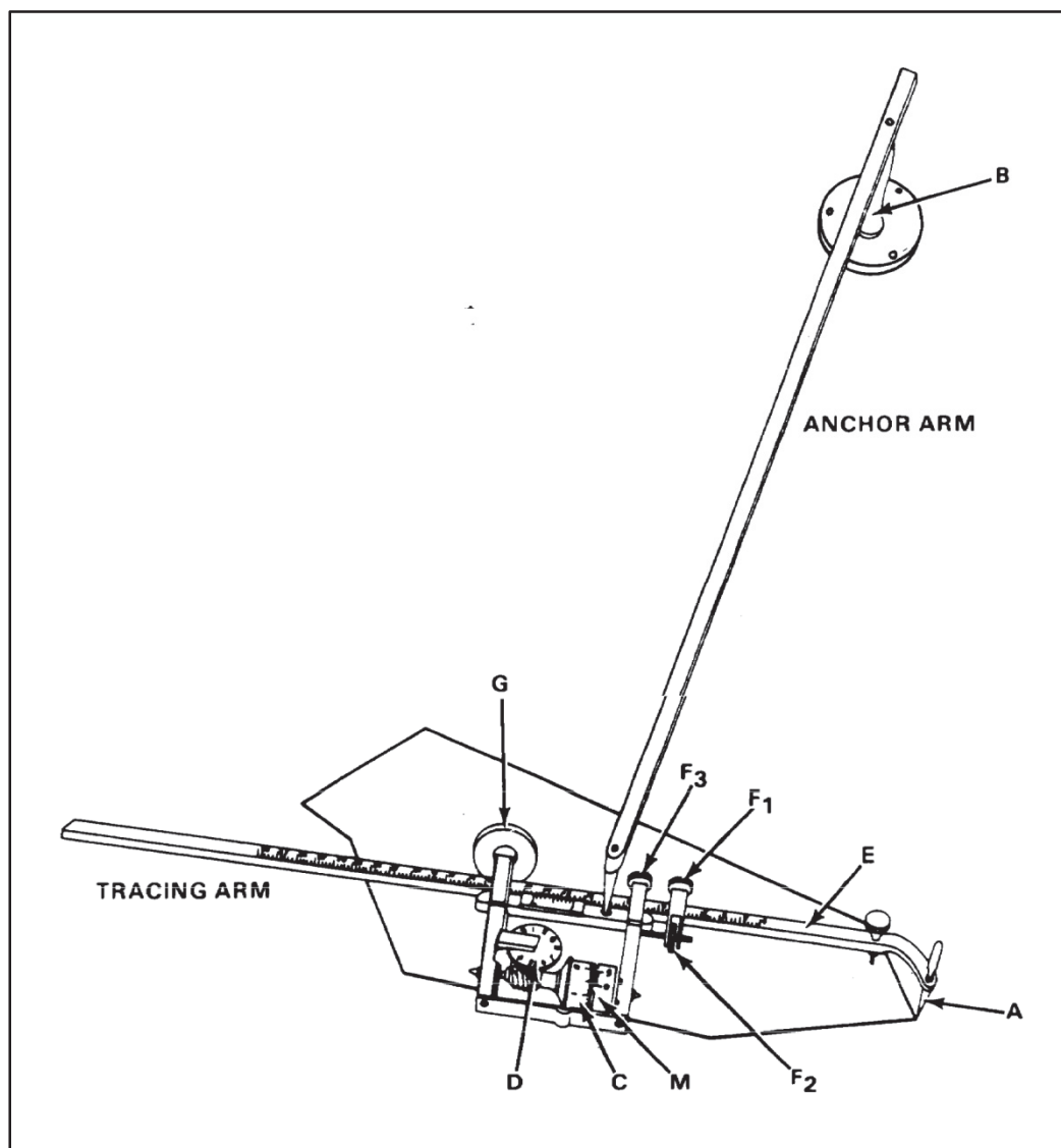
Figure 4-6. Polar planimeter
