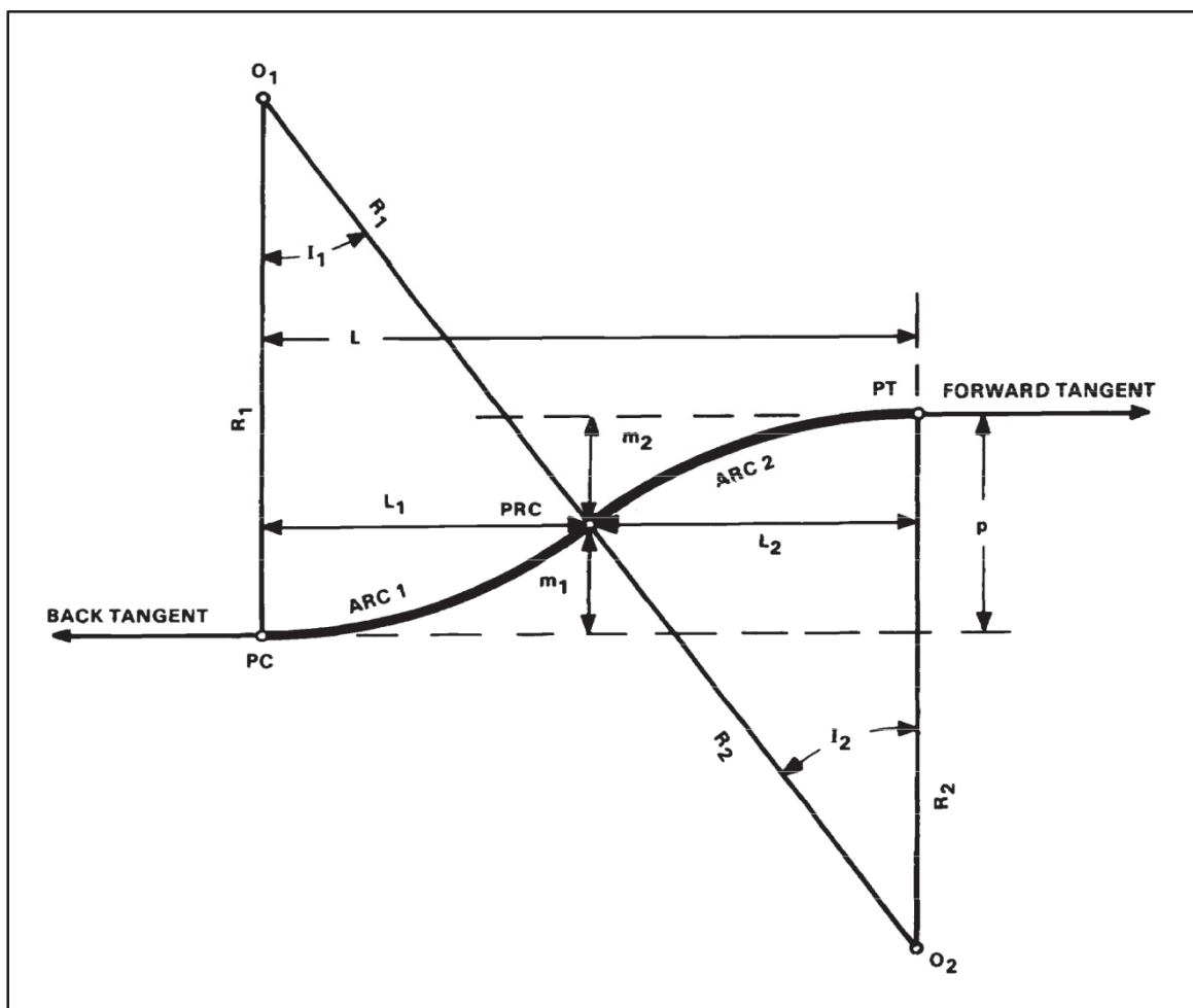
Figure 3-13. Reverse curve connecting parallel tangents
