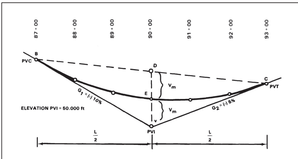
Figure 3-19. Grade lines connected by a vertical curve
