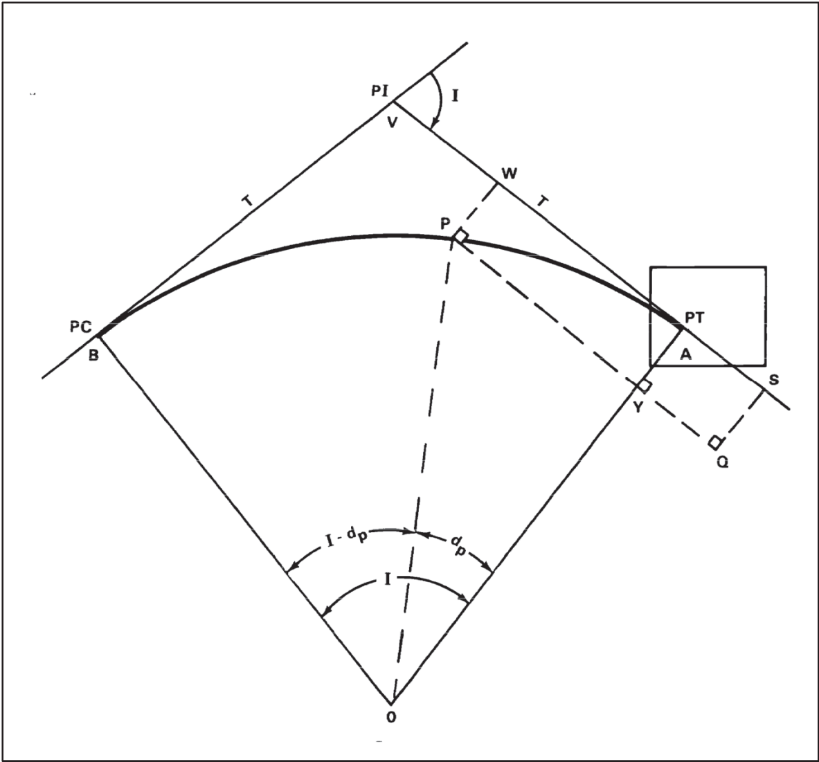
Figure 3-8. Inaccessible PT
