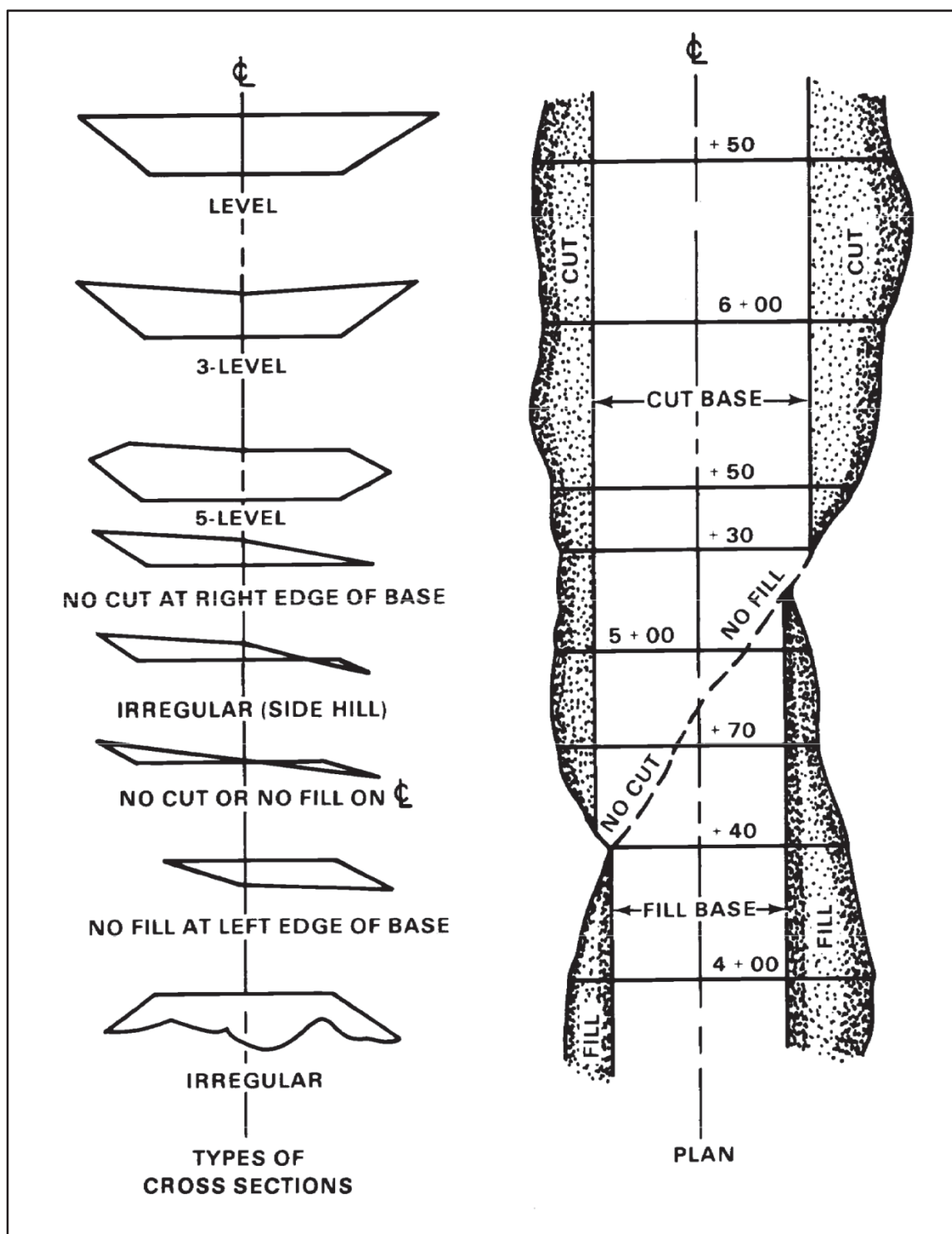
Figure 4-1. Typical cross sections
