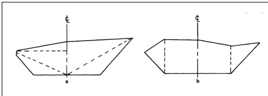
Figure 4-3. Subdividing cross sections
