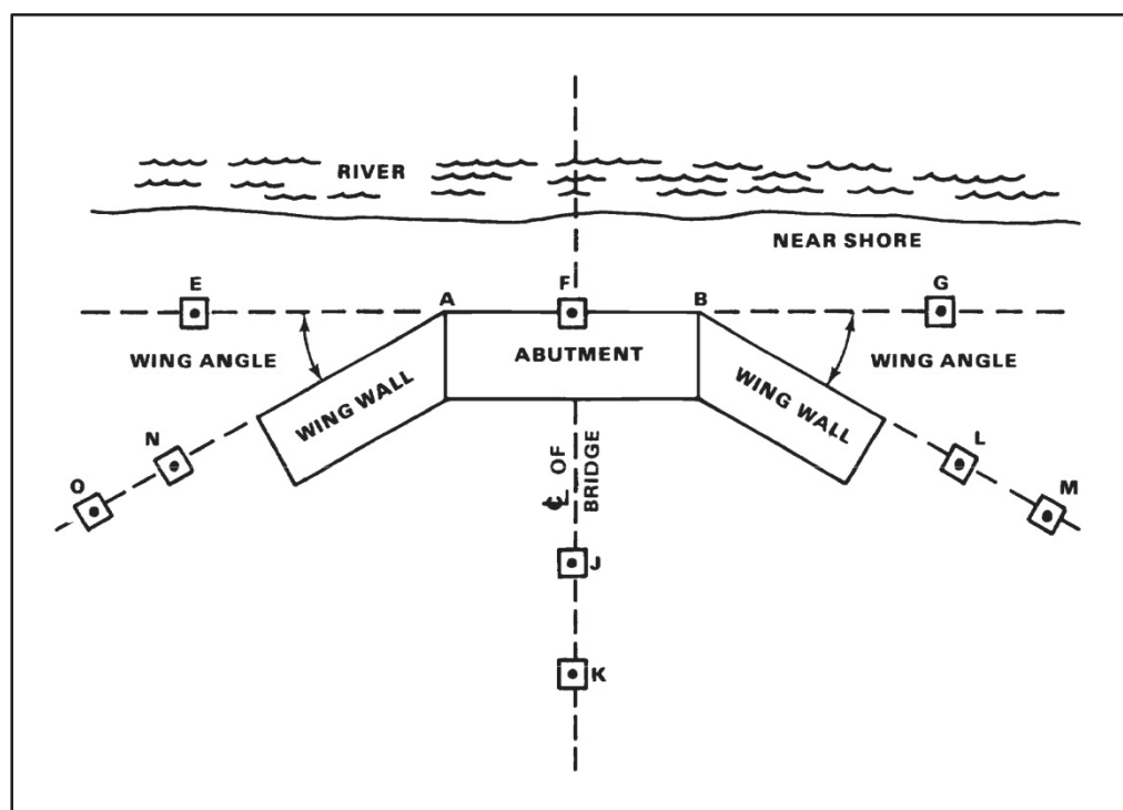
Figure 5-3. Staking wing walls
