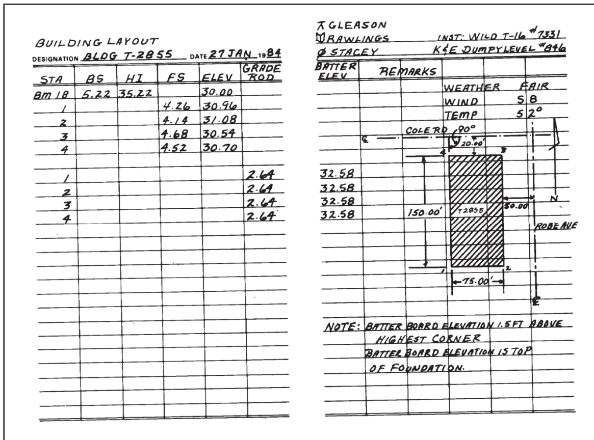
Figure B-14. Building layout
