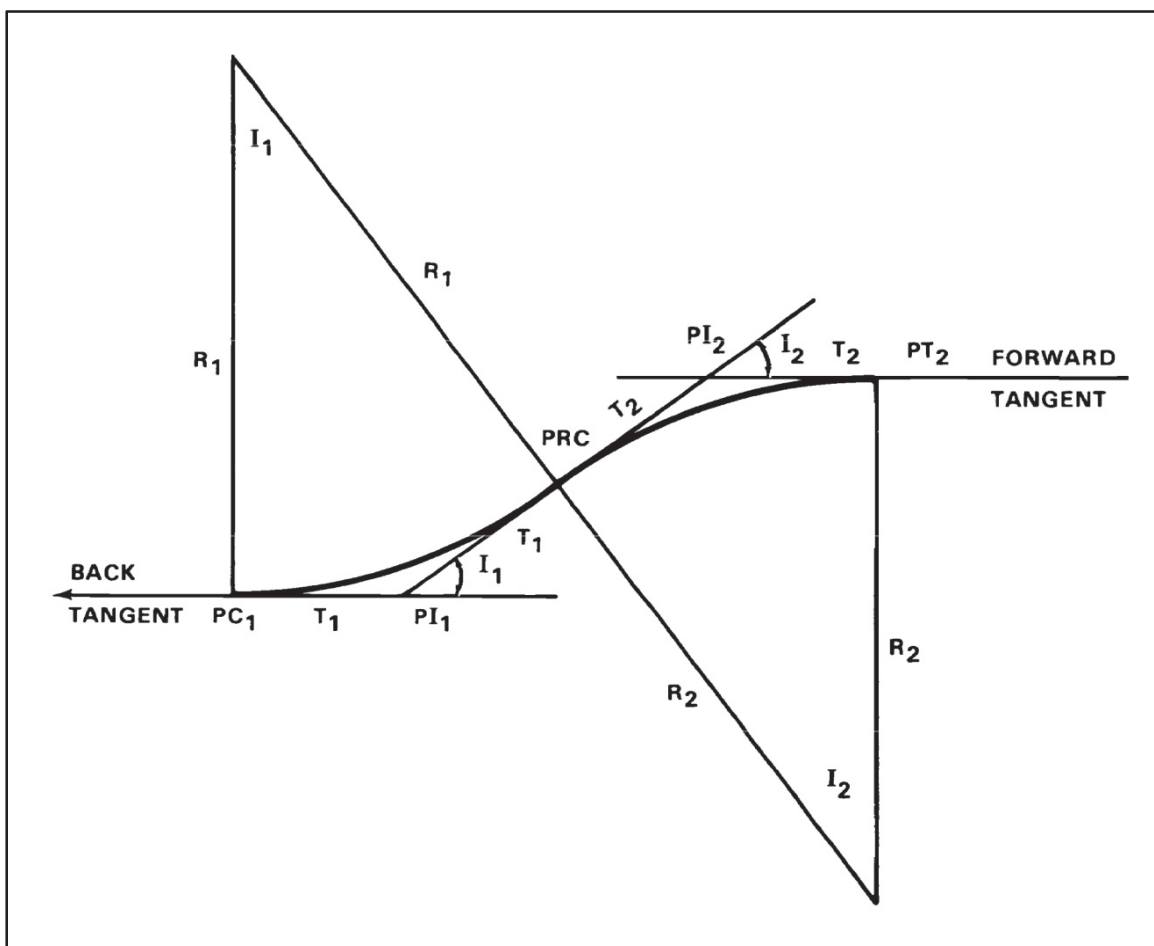
Figure 3-12. Reverse curve between successive PIs
