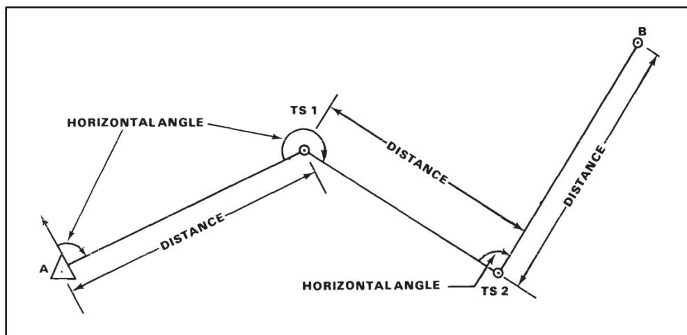
Figure 7-1. An open traverse
