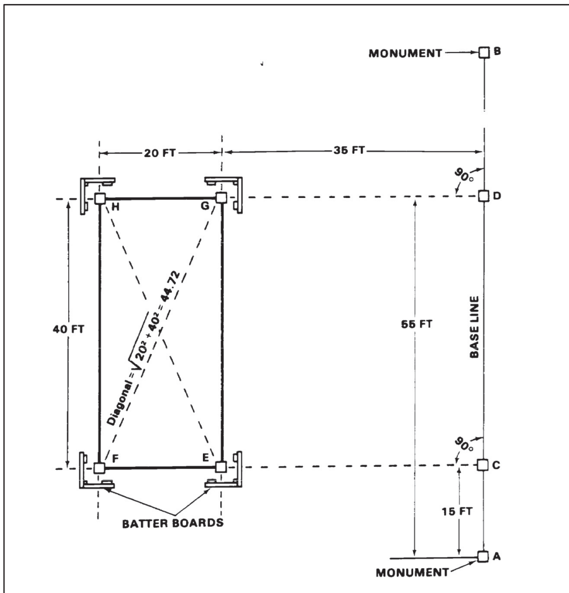
Figure 6-1. Building layout
