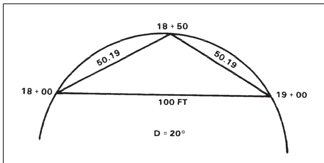
Figure 3-5. Subchord corrections
