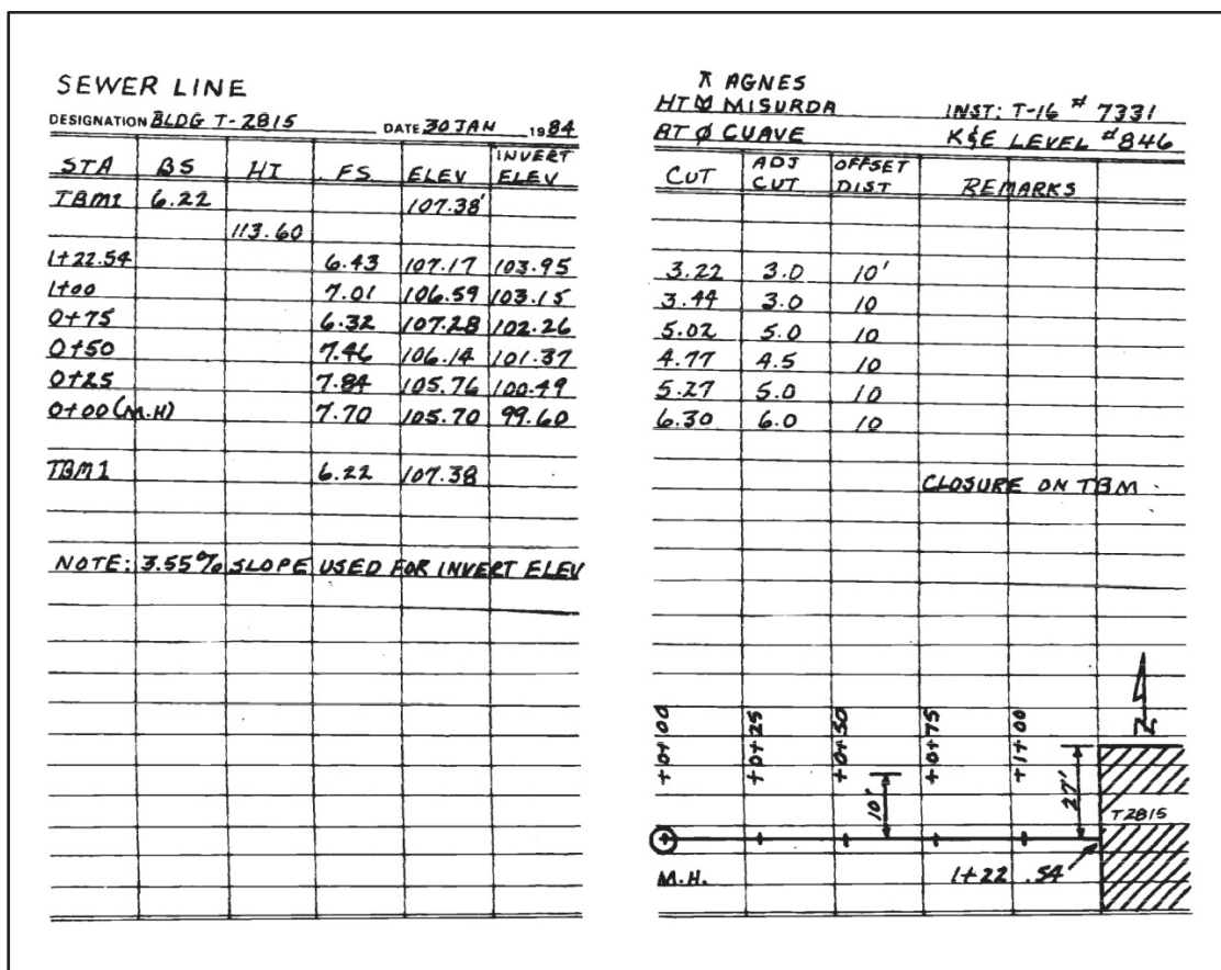
Figure B-15. Sewer line
