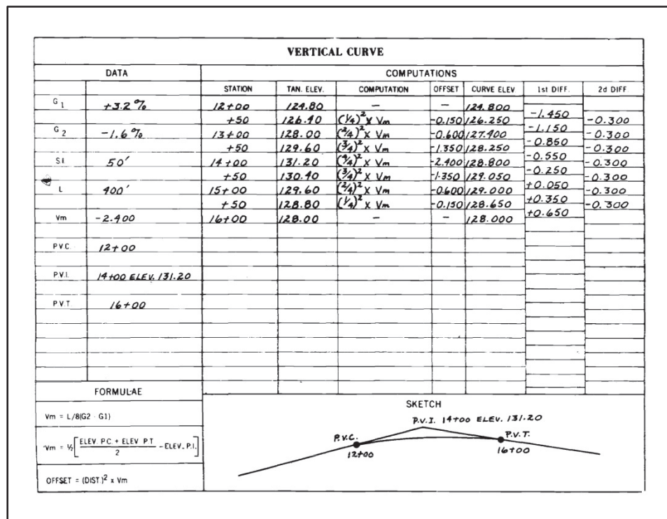
Figure 3-21. Typical solution of a summit curve
