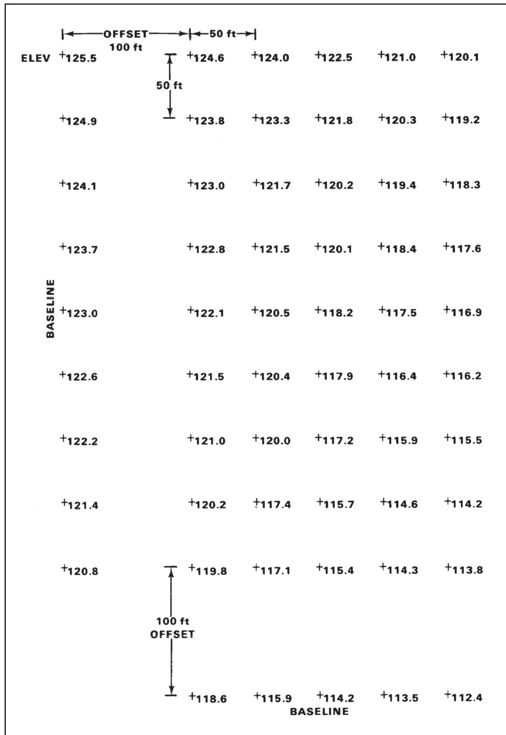
Figure 4-7. Typical grid layout for borrow pits
