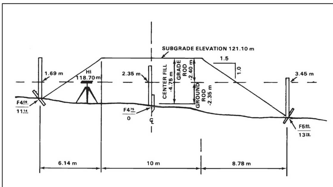
Figure 2-5. Slope stakes (HI below grade elevation)
