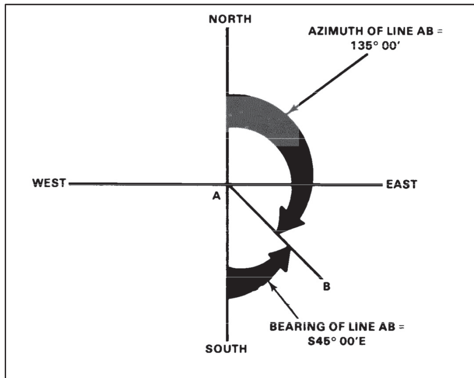
Figure 7-3. Relationship of azimuth and bearing
