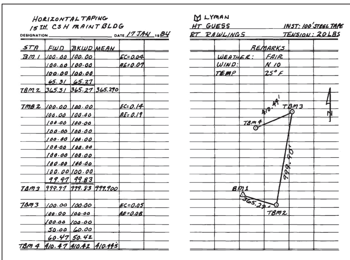
Figure B-5. Horizontal taping
