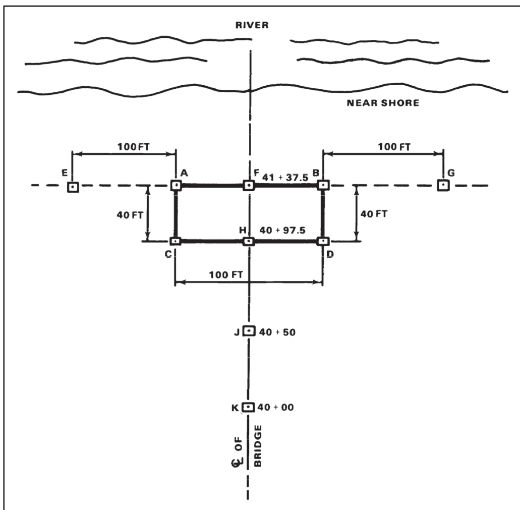
Figure 5-2. Staking an abutment
