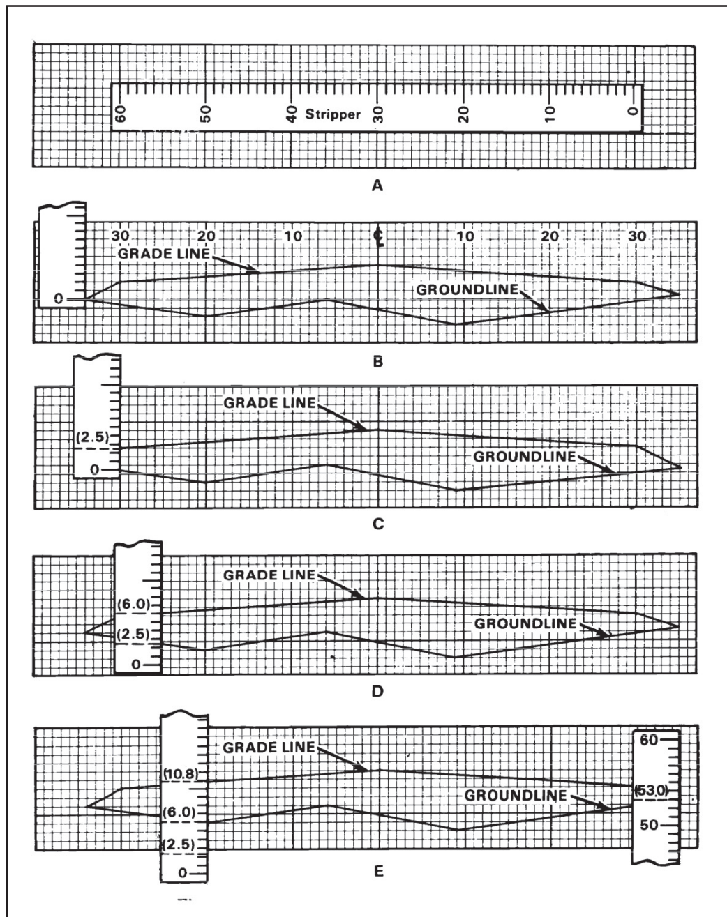
Figure 4-4. Cross-section area by stripper method
