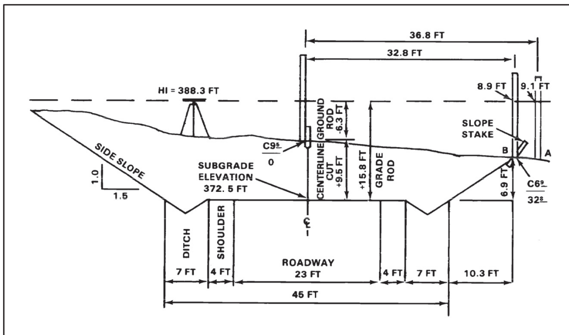
Figure 2-2. Setting slope stakes
