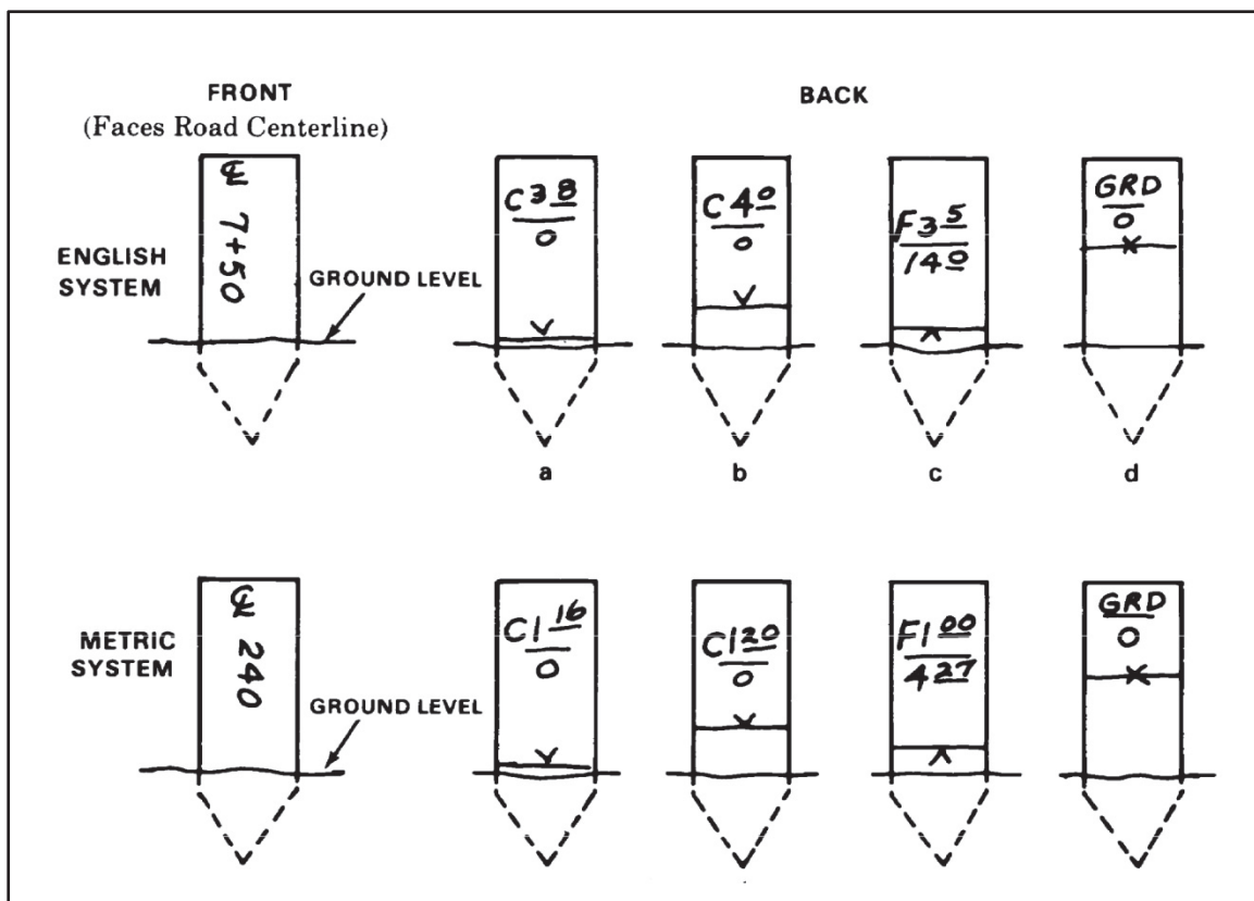
Figure 2-1. Grade stakes
