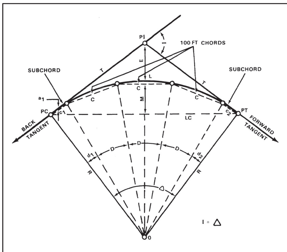
Figure 3-2. Elements of a simple curve
