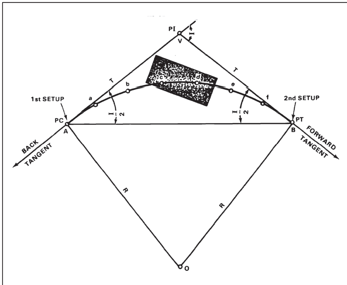
Figure 3-9. Obstacle on a curve
