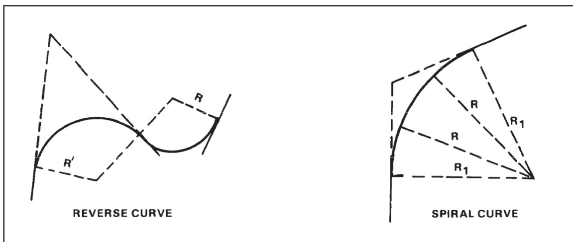
Figure 3-1. Horizontal curves (continued)
