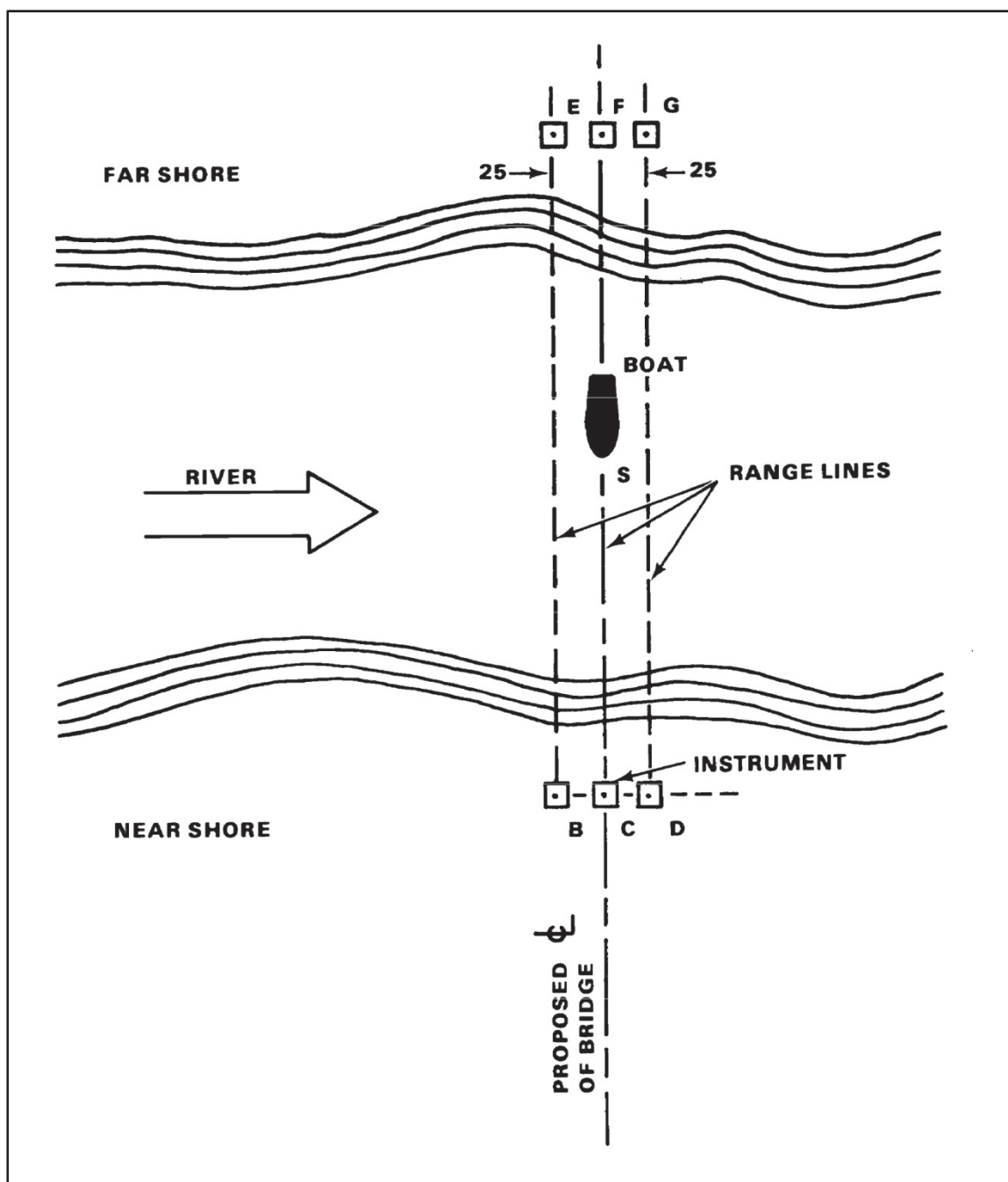
Figure 5-1. Taking soundings
