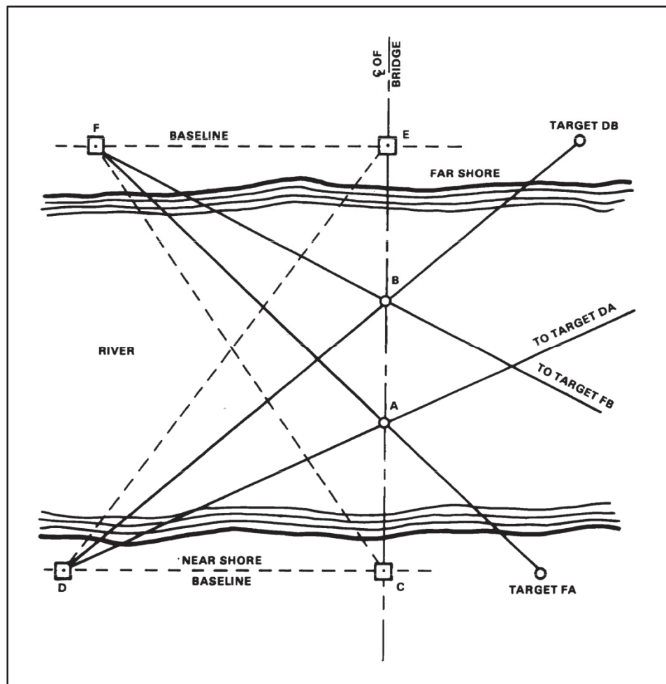
Figure 5-4. Locating piers
