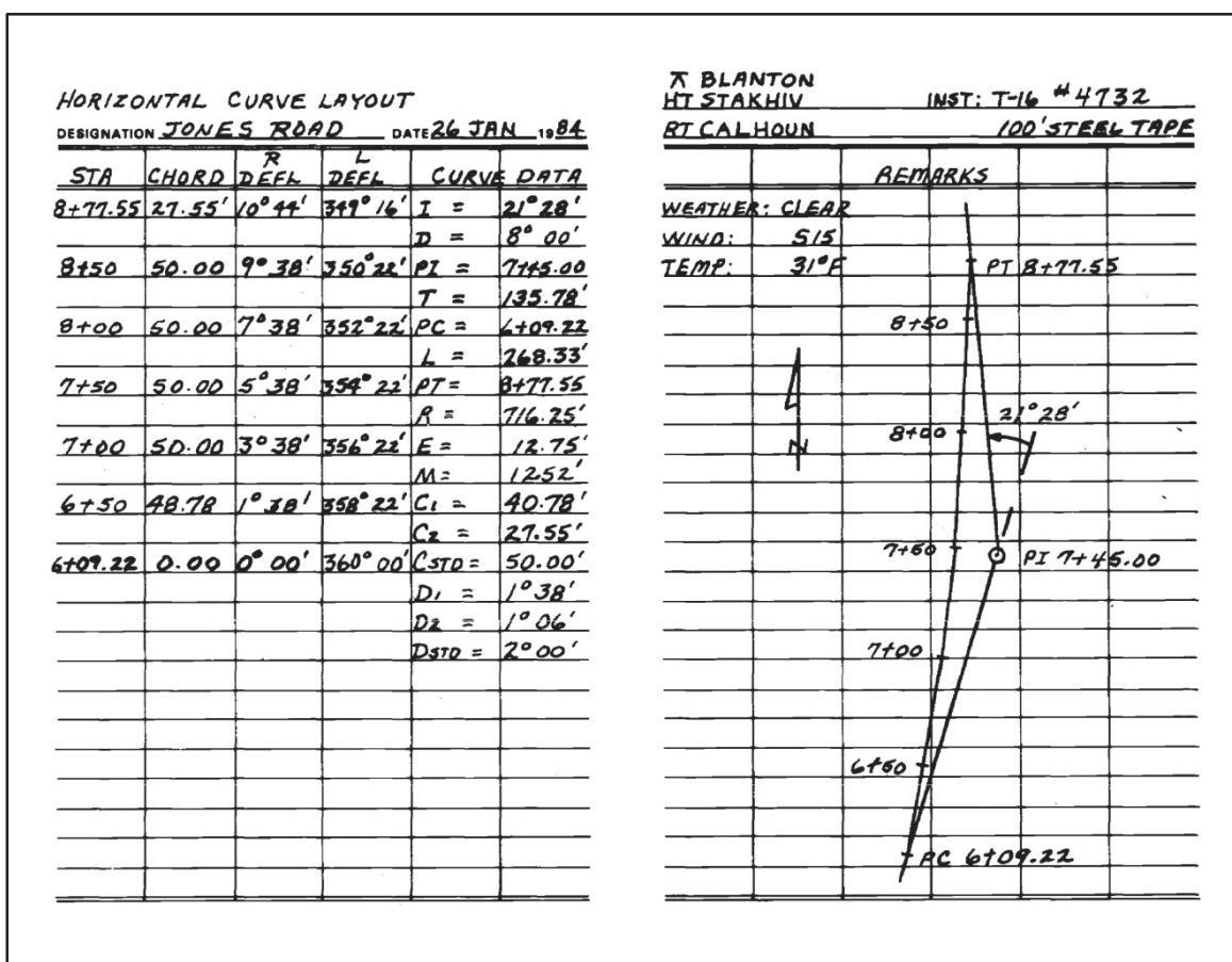
Figure B-13. Horizontal curve layout
