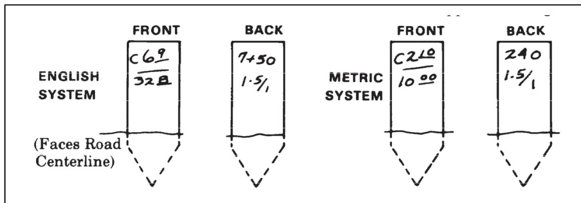
Figure 2-4. Slope stakes (HI above grade elevation)
