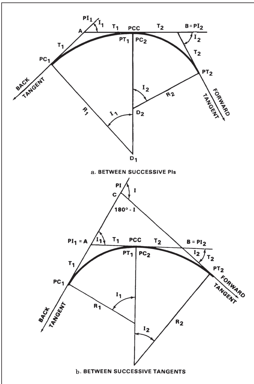
Figure 3-11. Compound curves
