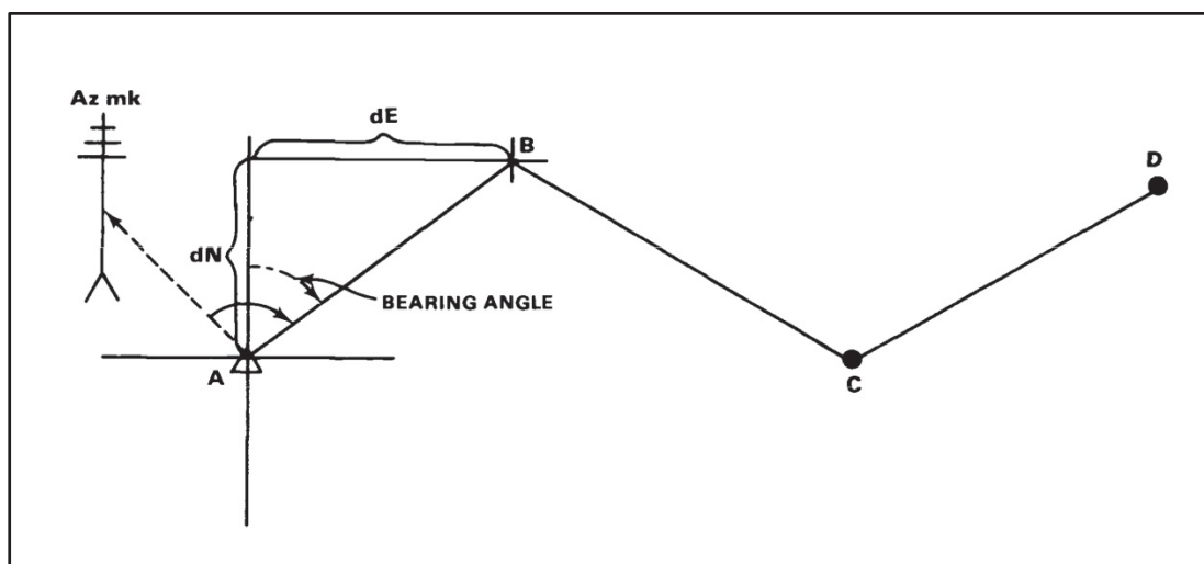
Figure 7-5. Requirements for dN and dE
