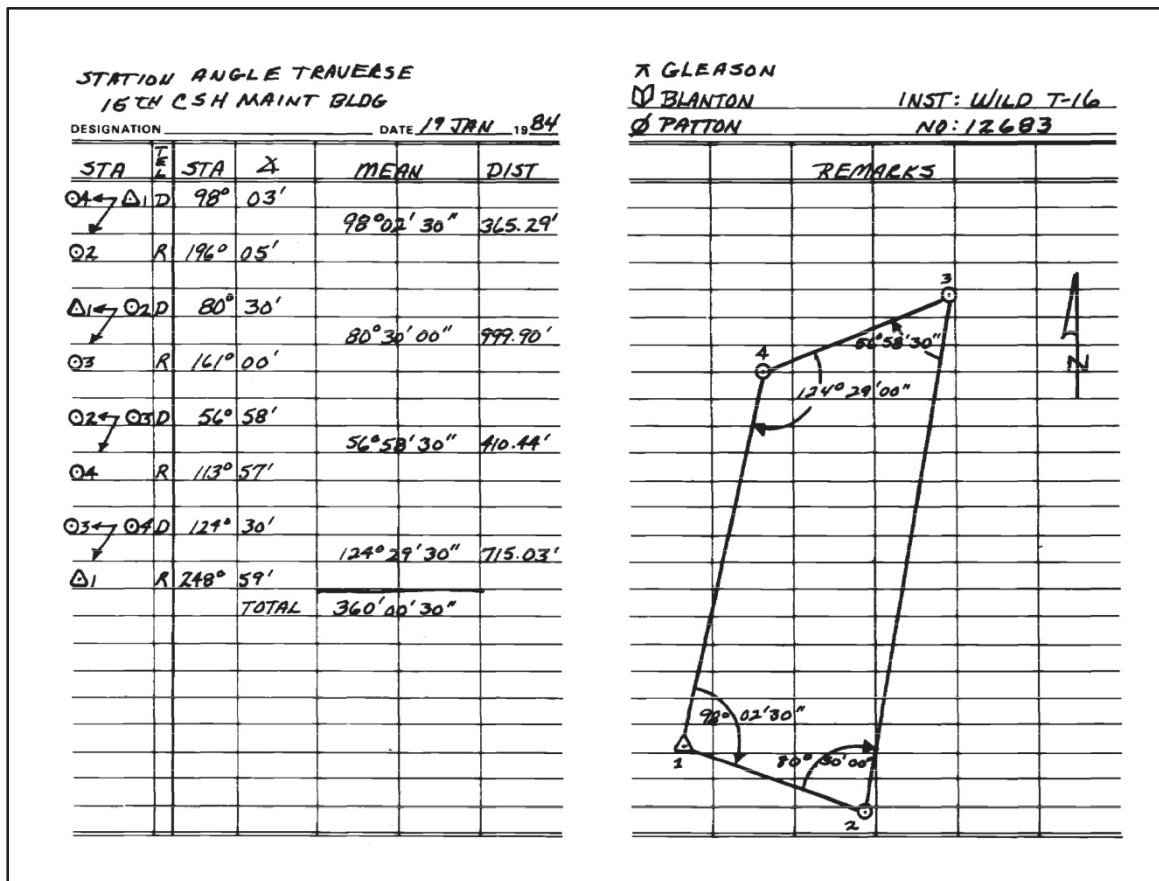
Figure B-6. Station angle traverse
