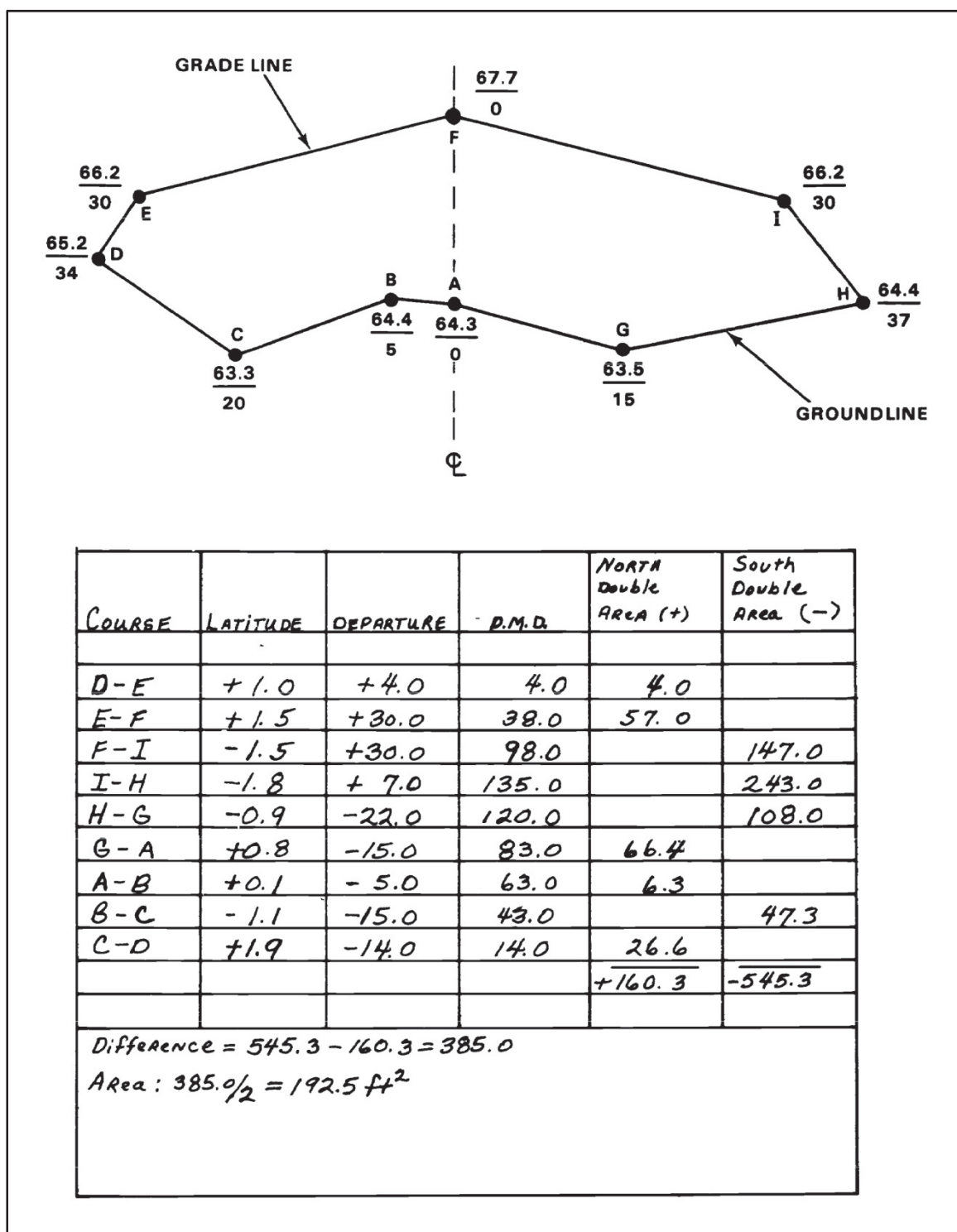
Figure 4-5. Cross-section area by double-meridian-distance method
