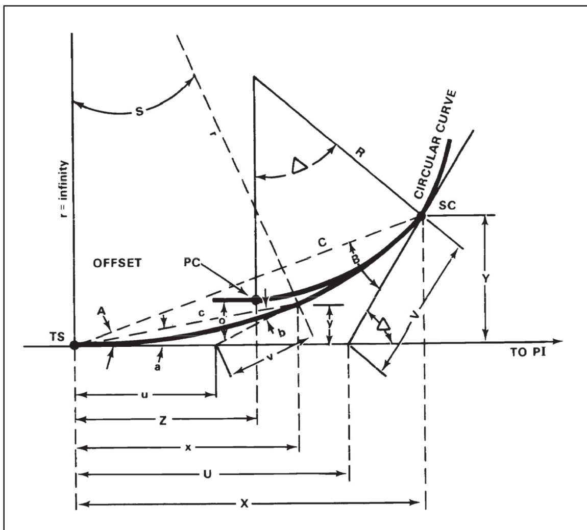
Figure 3-16. Enlargement of spiral of figure 3-15
