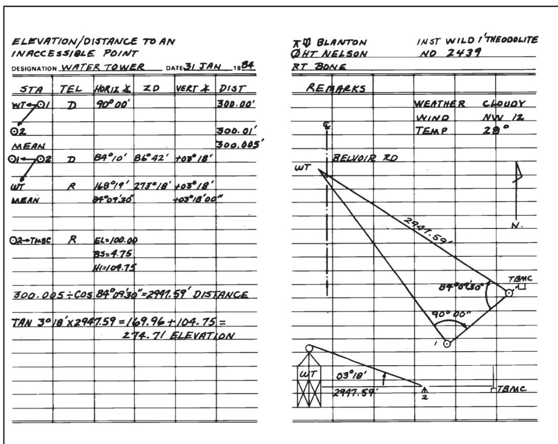
Figure B-17. Elevation/distance of an inaccessible point
