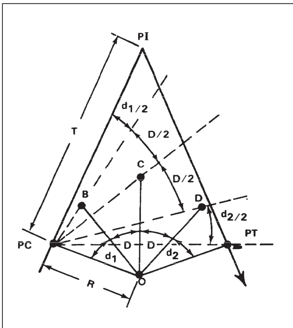
Figure 3-4. Deflection angles
