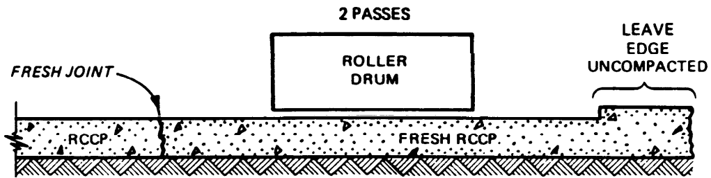
(3) ROLL REMAINING UNCOMPACTED RCCP REPEAT SEQUENCE
