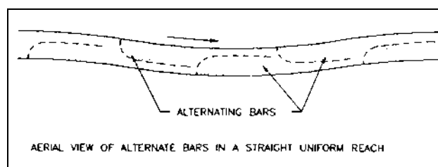
Figure B-1. Alternate bars
